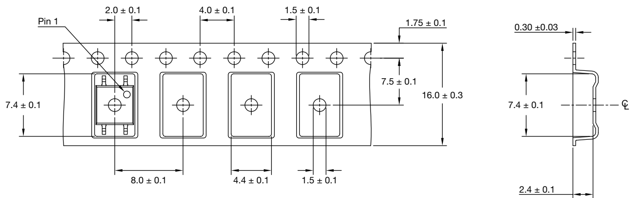
Fig. 16 - VO1400AEFT (3000 pieces on reel)
