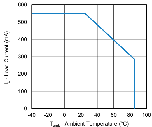
Fig. 3 - Load Current vs. Ambient Temperature
