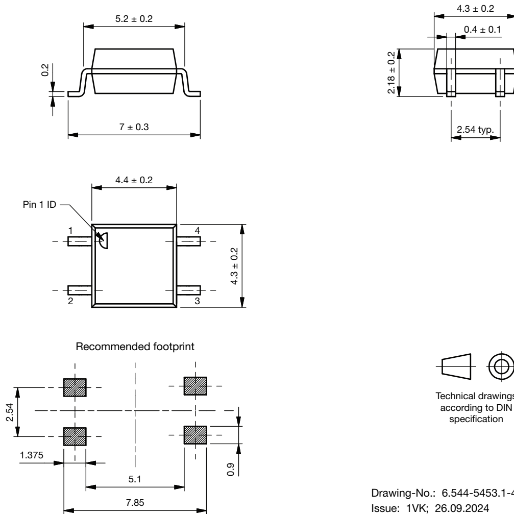
Fig. 14 - Package Drawings
