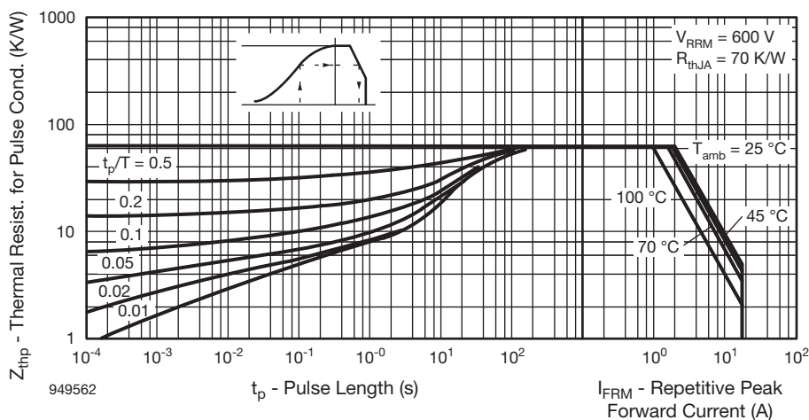
Fig. 7 - Thermal Response
