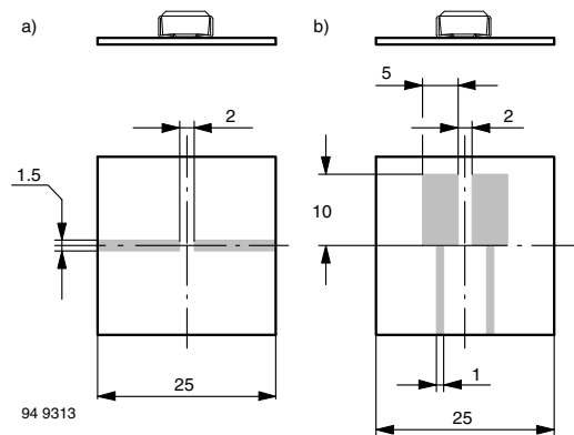
Fig. 1 - Boards for R_{thJA} Definition (Copper Overlay 35\text{ }\mu\text{m} )
