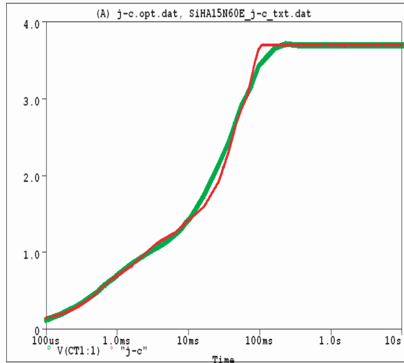
SiHA15N60E Tank j-c Temperature:27.0
