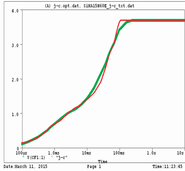
SiHA15N60E Filter j-c Temperature:27.0
