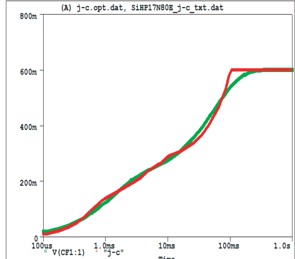
SiHP17N80E Filter j-c Temperature 27.0
