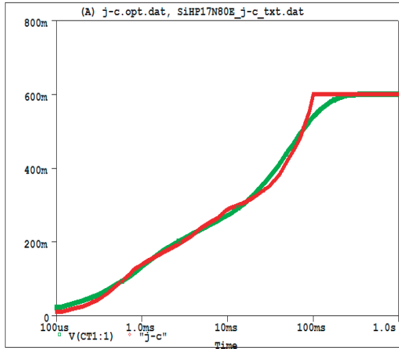
SiHP17N80E Tank j-c Temperature 27.0
