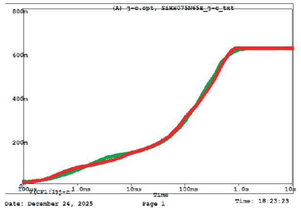
SiHH075N65E Filter j-c Temperature: 27.0
