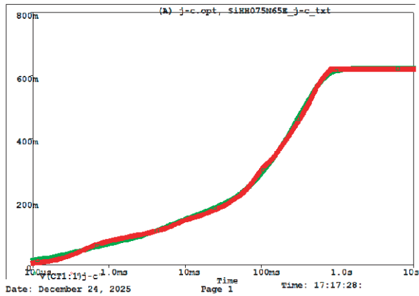
SiHH075N65E Tank j-c Temperature: 27.0
