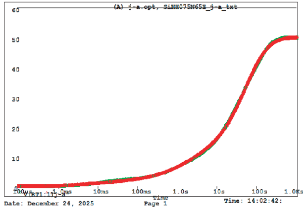
SiHH075N65E Tank j-a Temperature: 27.0
