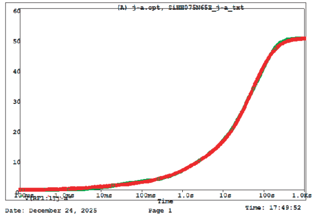
SiHH075N65E Filter j-a Temperature: 27.0
