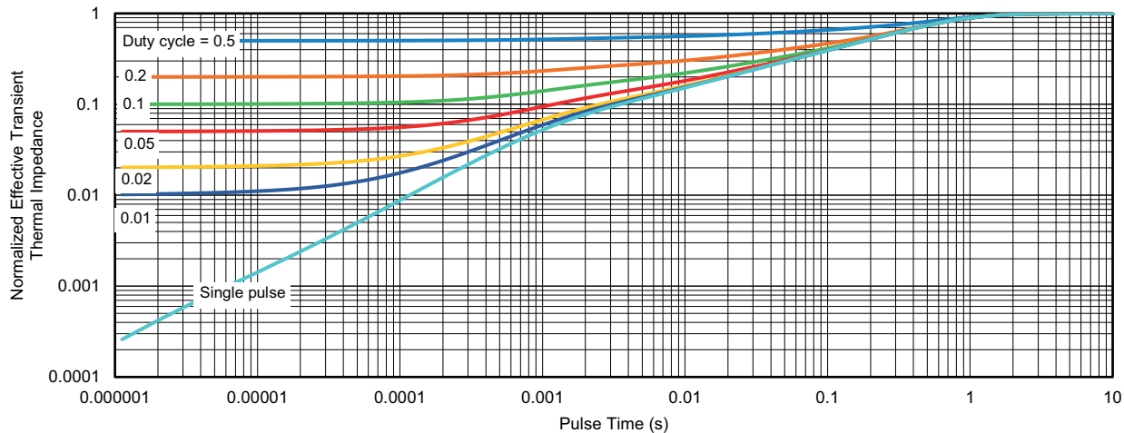
Fig. 12 - Normalized Transient Thermal Impedance, Junction-to-Case
