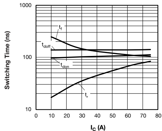
Fig. 26 - Typical Q2 - Q3 Trench IGBT Switching Time vs. I_C (with F/W External TO-247 Diode Discrete 30ETH06), T_J = 125\text{ }^\circ\text{C} , V_{CC} = 300\text{ V} , R_g = 4.7\ \Omega , V_{GE} = 15\text{ V} , L = 500\ \mu\text{H}
