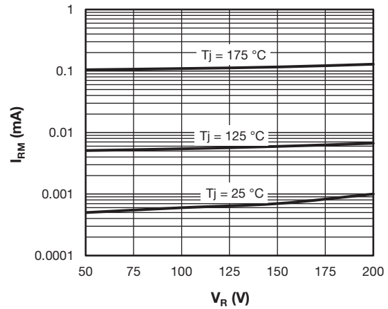
Fig. 13 - Typical Chopper Diode Reverse Leakage Current
