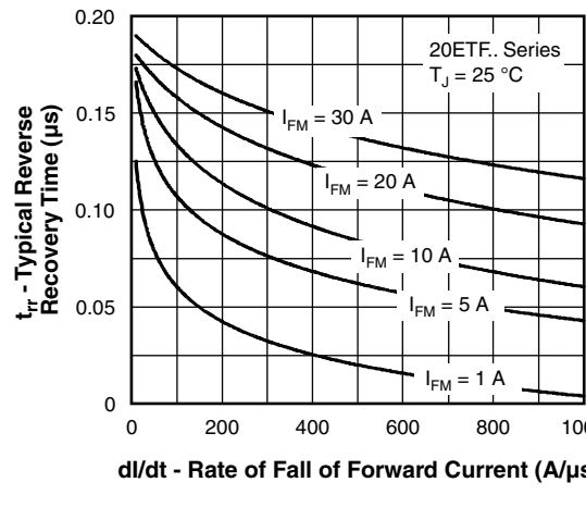
Fig. 8 - Recovery Time Characteristics, Tj = 25 °C
