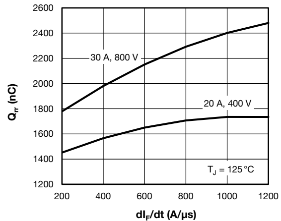
Fig. 8 - Typical Reverse Recovery Time vs. dl_F/dt , Per Leg
