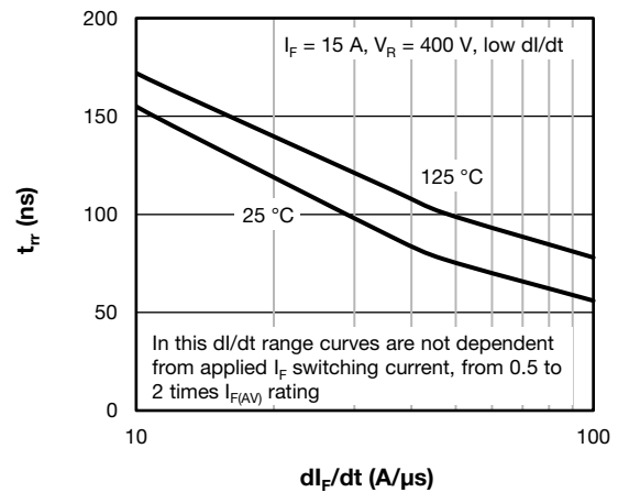
Fig. 10 - Typical Recovery Time vs. dI_F/dt , Per Leg
