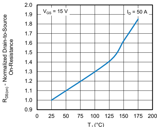
Fig. 4 - Normalized Drain-to-Source On-Resistance vs. Temperature
