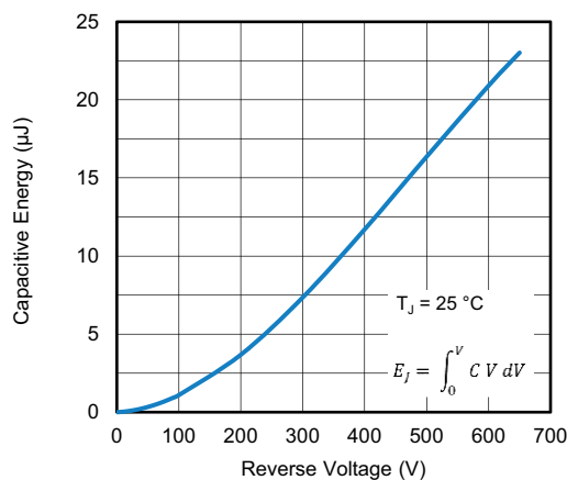
Fig. 8 - Capacitance Energy vs. Reverse Voltage Per Leg
