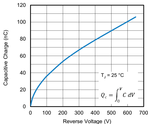
Fig. 9 - Capacitance Change vs. Reverse Voltage Per Leg
