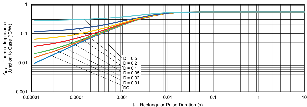
Fig. 5 - Thermal Impedance Z_{thJC} - Characteristics Per Leg
