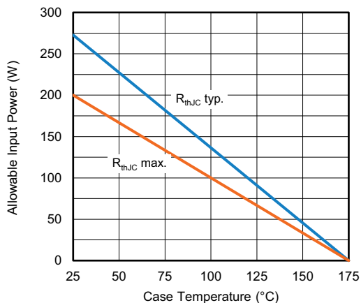
Fig. 7 - Allowable Input Power vs. Case Temperature Per Leg
