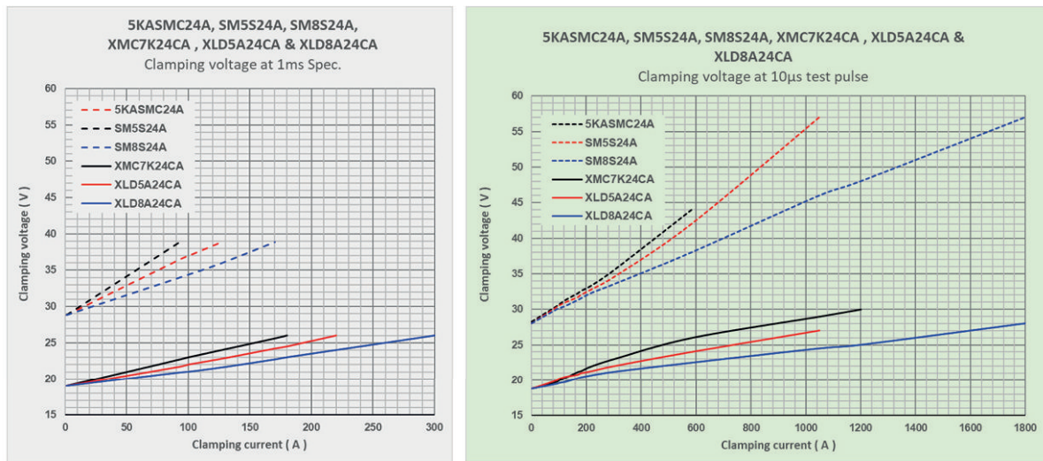
Fig. 1-5: Clamping Voltages of XClamp TVS and Conventional TVS
