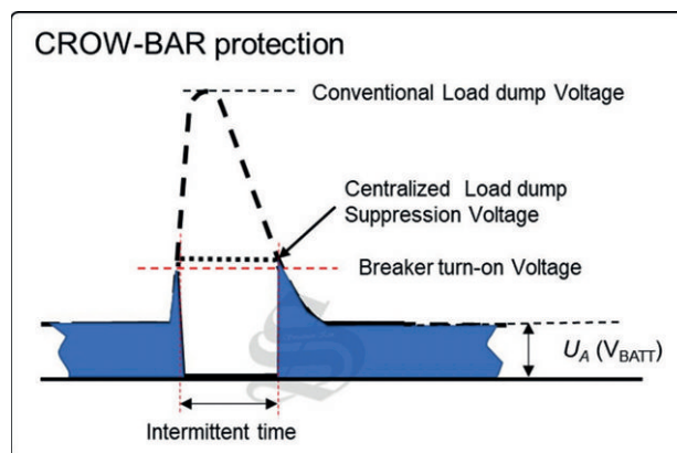
Fig. 1-10: Crow-bar Protection
