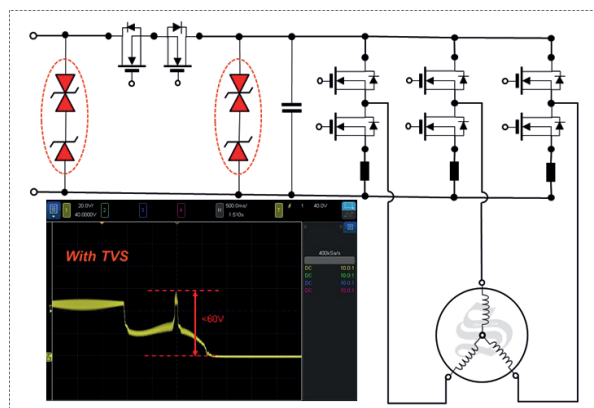
Fig. 2-3C: XMC7K24CA and 5KASMC28A Combination in a Motor Drive Circuit with Waveform
