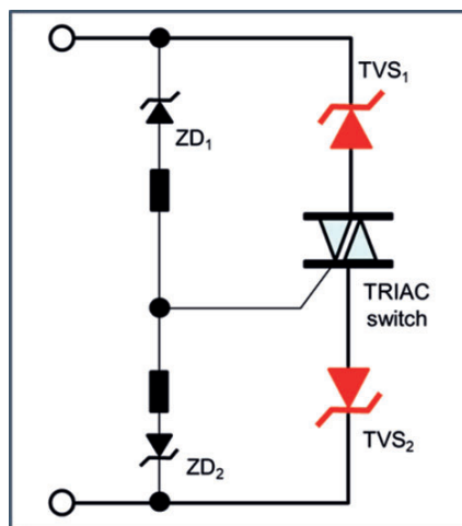
Fig.1-2: Schematic Circuit of XClamp TVS
