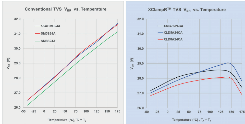
Fig. 1-8: Breakdown Voltages of Conventional TVS and XClampR TVS
