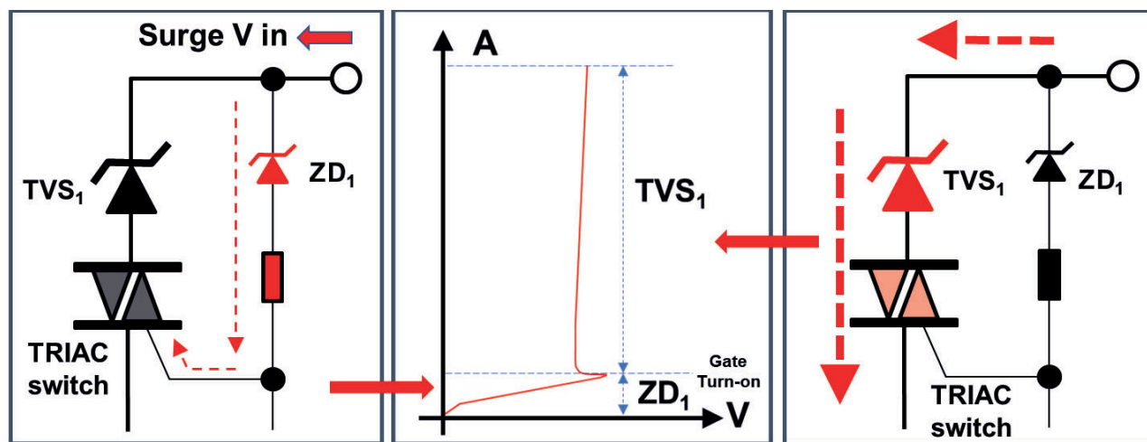
Fig.1-3: Operation Concept of XClamp TVS
