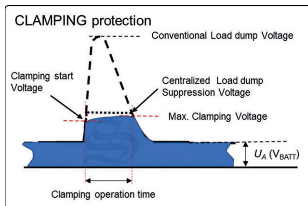
Fig. 1-9: Clamping Protection
