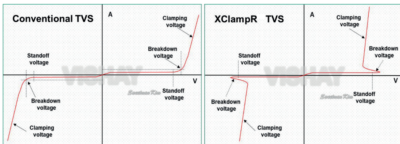
Fig.1-1: I-V Curve of Conventional Bidirectional TVS and XClamp TVS
