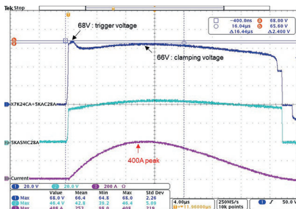
Fig. 2-3D: XMC7K24CA and 5KASMC28A Combination at a 400 A, 8/20 \mu s Pulse Width
