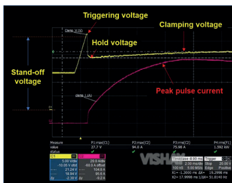
Fig. 1-4: Operating of XLD8A24CA at ISO 16750-2 101 V U_S , 12 V U_A , 400 ms Pulse Width and 0.75 \Omega R_i
