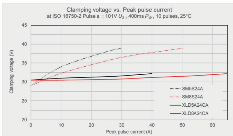
Fig.2-3: Clamping Voltage vs. Peak Pulse Current
