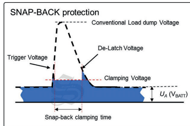
Fig. 1-11: Snap-back Protection
