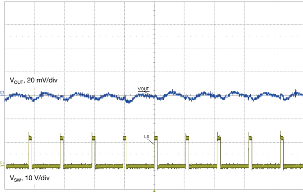
Fig. 36 - Output Ripple, 0.1 A, t = 2\ \mu\text{s}/\text{div} Forced Continuous Conduction Mode
