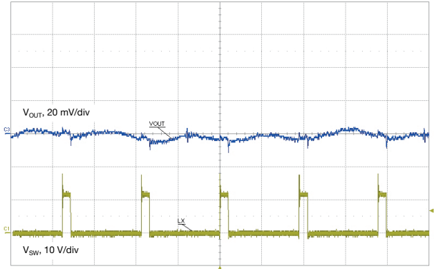
Fig. 38 - Output Ripple, 12 A, t = 1\ \mu\text{s}/\text{div} Forced Continuous Conduction Mode
