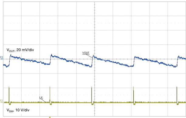
Fig. 37 - Output Ripple, 0.1 A, t = 20\ \mu\text{s}/\text{div} Skip Mode Enabled
