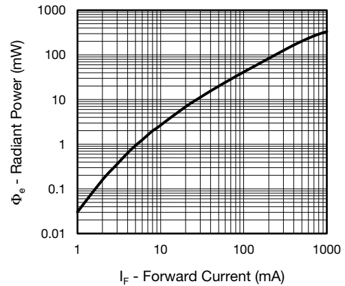
Fig. 3 - Radiant Power vs. Forward Current (pulsed t p = 300 μs, t p /T = 0.001)
