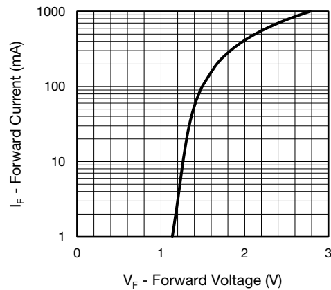
Fig. 4 - Forward Current vs. Forward Voltage (pulsed t p = 300 μs, t p /T = 0.001)
