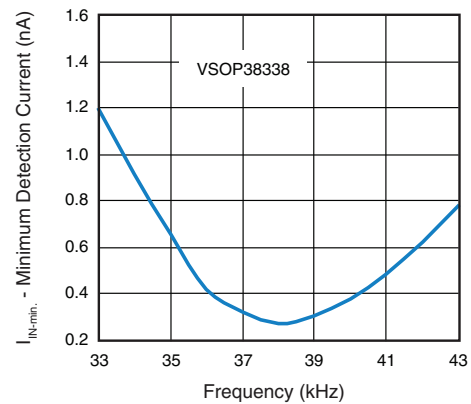
Fig. 4 - Bandpassfilter Characteristic
