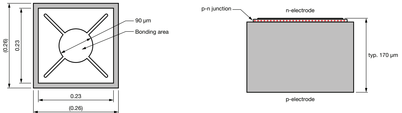
Fig. 3 - Sectional View
