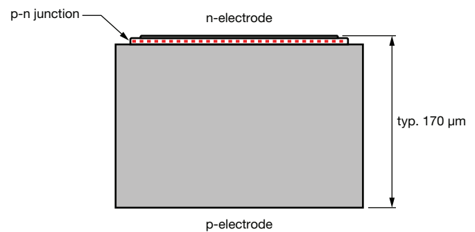
Fig. 3 - Sectional View
